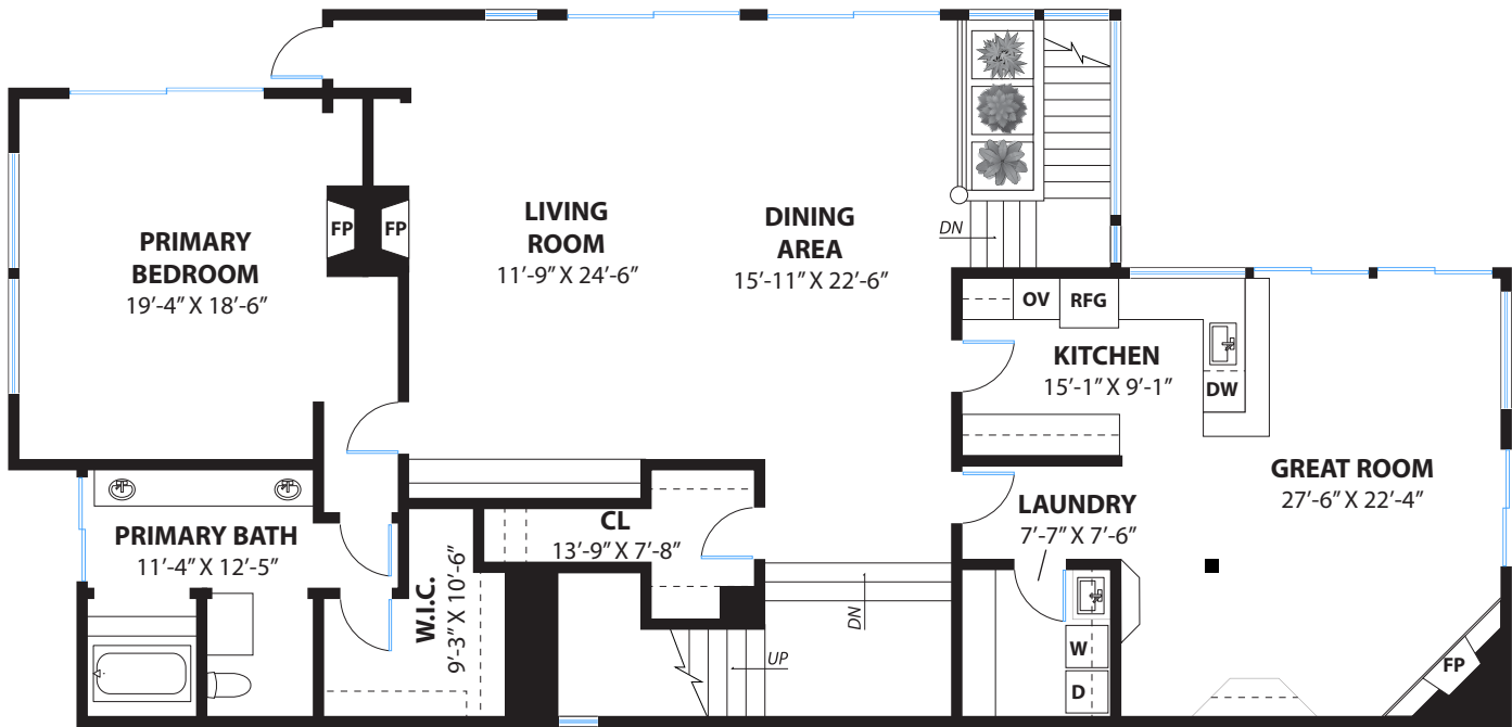
MAIN LEVEL
