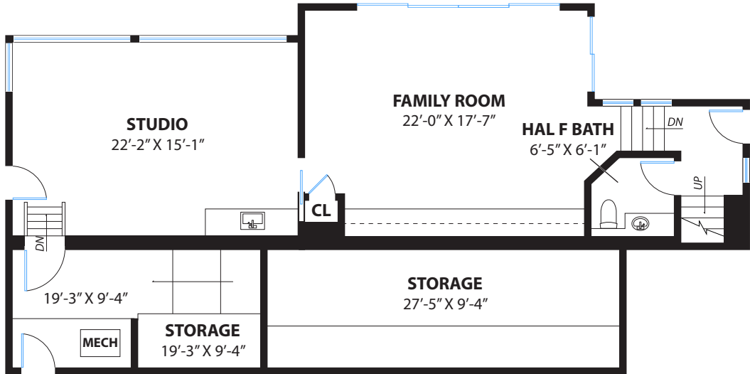
LOWER LEVEL
